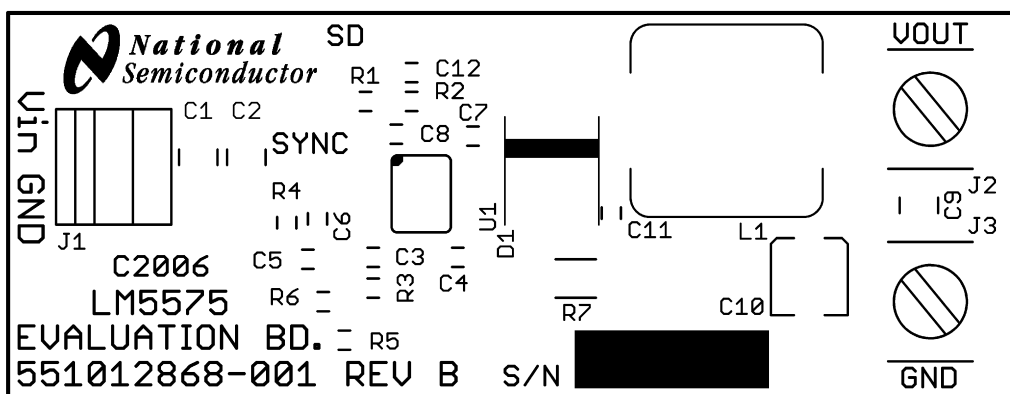
Figure 24. Silkscreen
