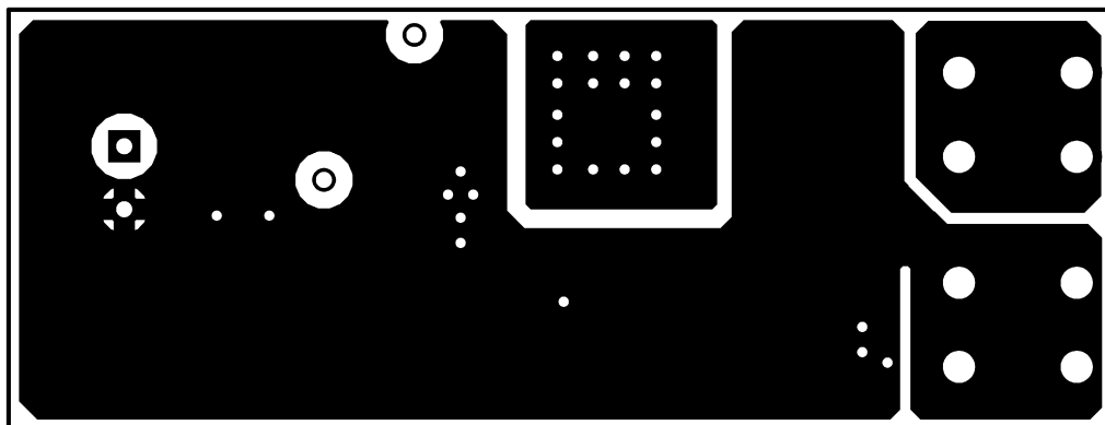
Figure 23. Solder Side
