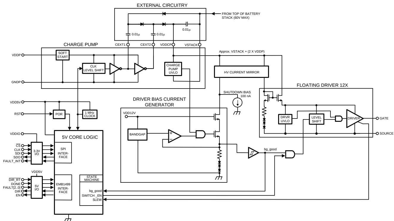
Figure 2. EMB1428 High-Level Block Diagram
