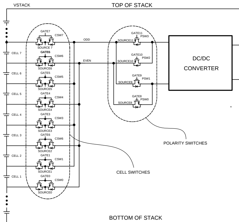
Figure 3. Switch Matrix
