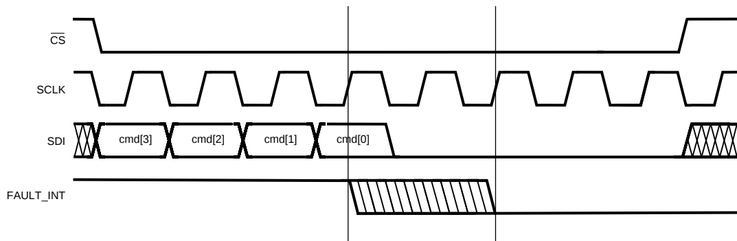
Figure 17. Clearing FAULT_INT
