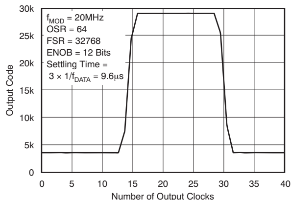
Figure 47. Pole Response of the Sinc 3 Filter
