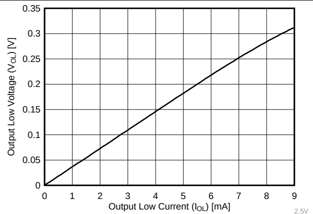
Figure 4. Typical Output Low Voltage of 2.5 V (25°C)
