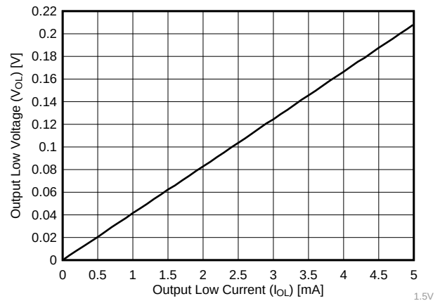
Figure 2. Typical Output Low Voltage of 1.5 V (25°C)
