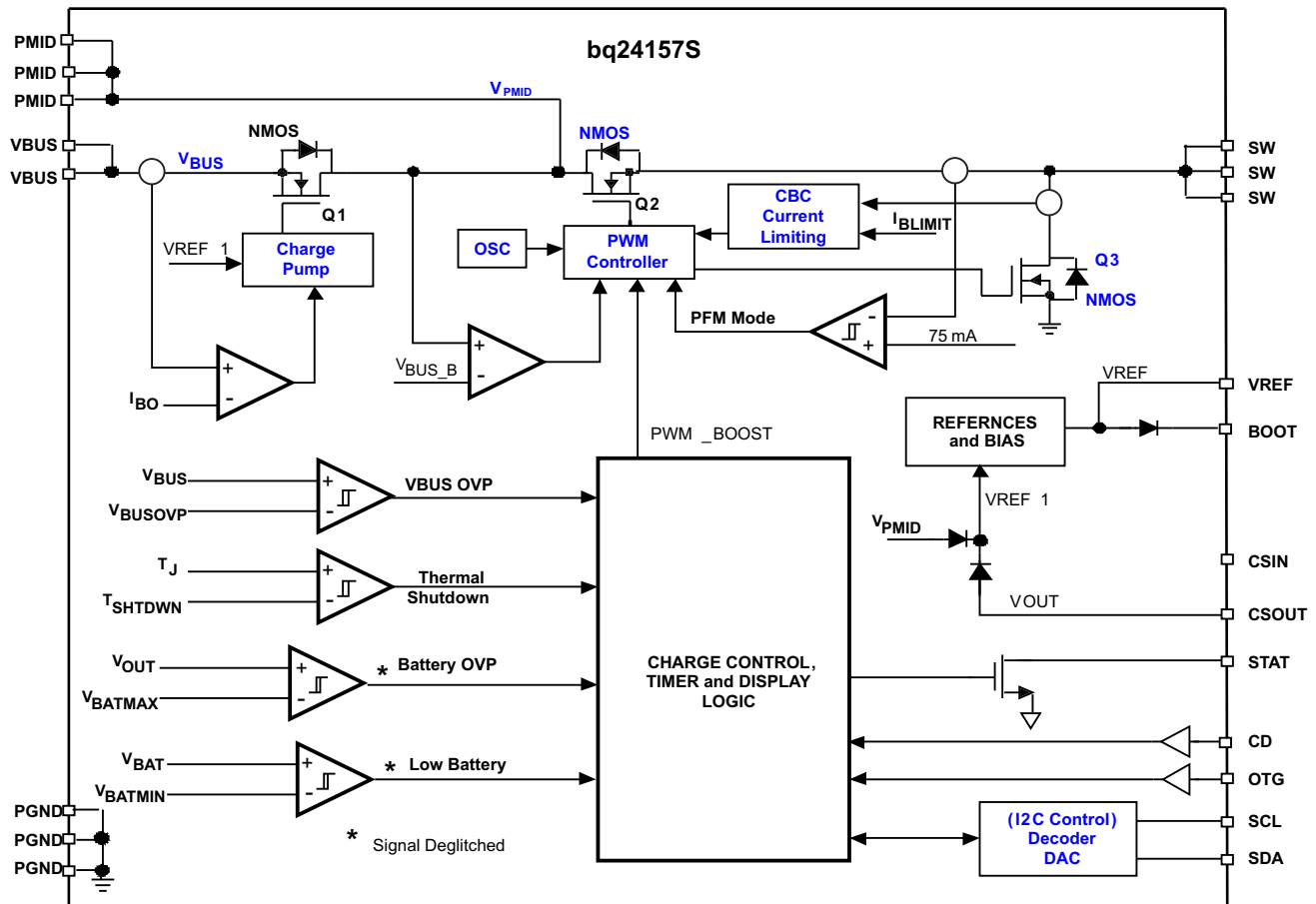
Figure 18. Function Block Diagram of bq24157S in Boost Mode
