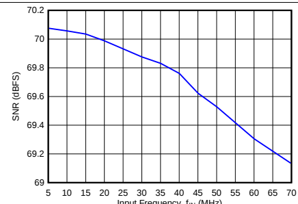
Figure 11. Signal-to-Noise Ratio vs f_{IN} in 10-Bit, 8-Input Mode
