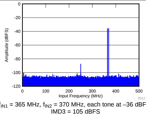
Figure 14. FFT for Two-Tone Input Signal (-36 dBFS)
