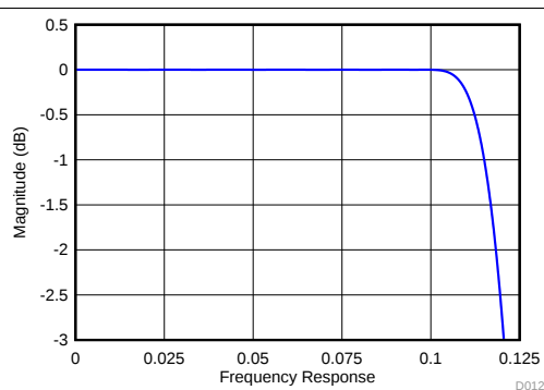
Figure 66. Decimate-by-4 with IQ Outputs Filter Response (Zoomed)
