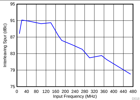
Figure 21. IL Spur vs Input Frequency
