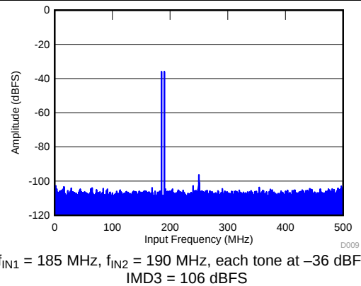
Figure 12. FFT for Two-Tone Input Signal (-36 dBFS)
