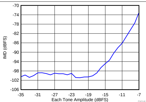
Figure 17. Intermodulation Distortion vs Input Tone Amplitude
