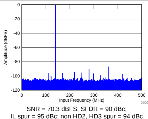
Figure 4. FFT for 140-MHz Input Signal
