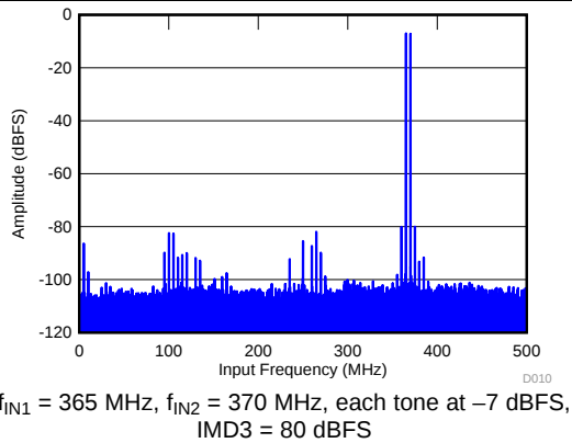
Figure 13. FFT for Two-Tone Input Signal (-7 dBFS)
