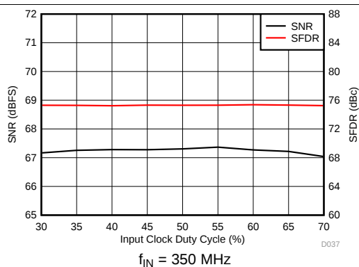
Figure 43. Performance vs Clock Duty Cycle
