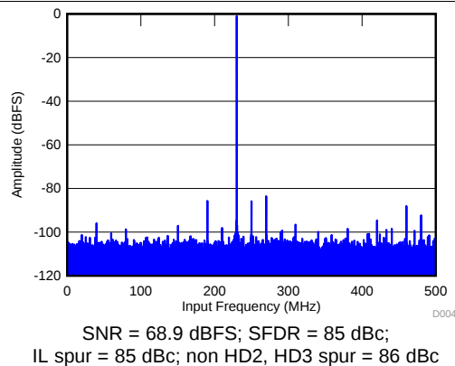
Figure 6. FFT for 230-MHz Input Signal
