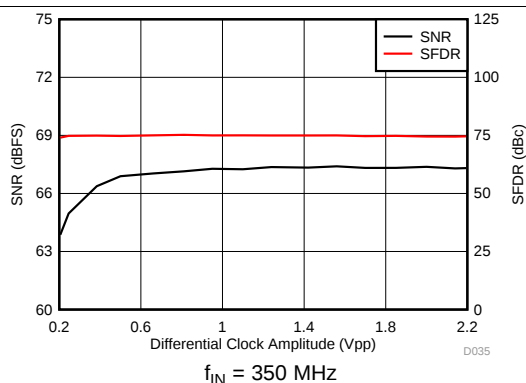
Figure 41. Performance vs Sampling Clock Amplitude
