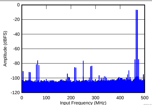
Figure 15. FFT for Two-Tone Input Signal (-7 dBFS)
