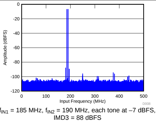
Figure 11. FFT for Two-Tone Input Signal (-7 dBFS)
