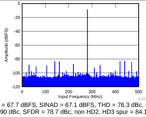
Figure 10. FFT for 720-MHz Input Signal at -6 dBFS
