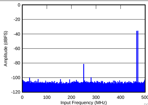
Figure 16. FFT for Two-Tone Input Signal (-36 dBFS)
