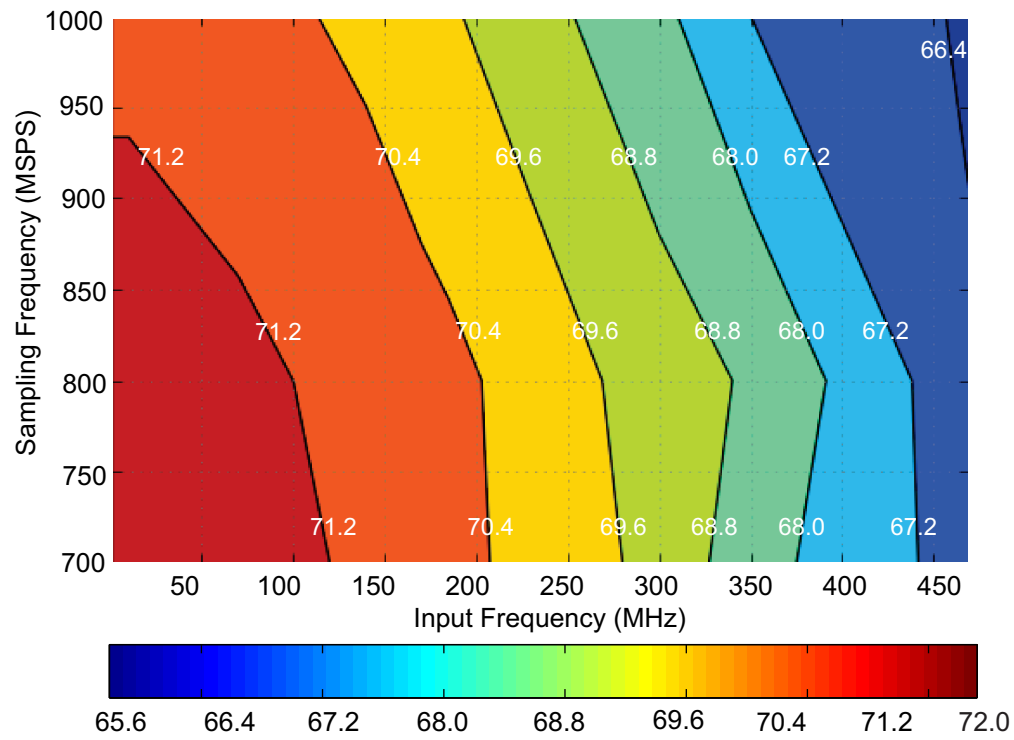
Figure 57. Signal-to-Noise-Ratio
