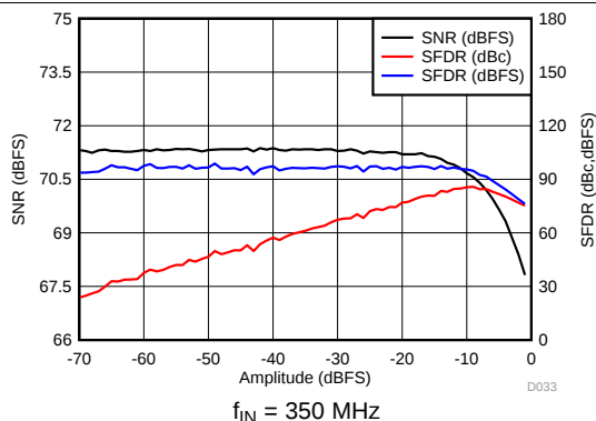
Figure 39. Performance vs Input Amplitude
