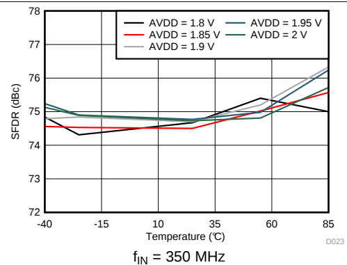
Figure 26. Spurious-Free Dynamic Range vs AVDD Supply and Temperature
