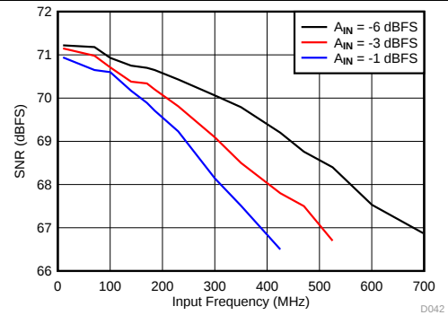
Figure 22. Signal-to-Noise Ratio vs Input Frequency
