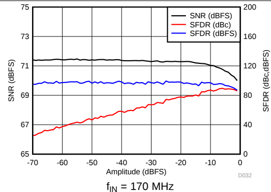
Figure 38. Performance vs Input Amplitude
