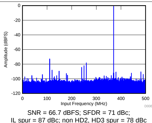
Figure 8. FFT for 370-MHz Input Signal
