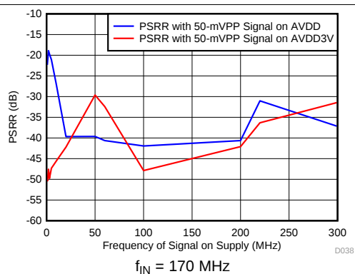
Figure 44. Power-Supply Rejection Ratio vs Test Signal Frequency
