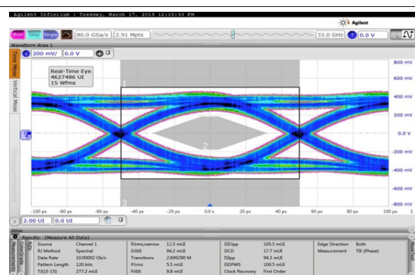
Figure 82. Eye at 10-Gbps Bit Rate with Increased Output Swing
