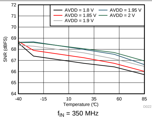
Figure 25. Signal-to-Noise Ratio vs AVDD Supply and Temperature
