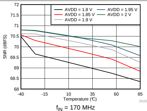
Figure 23. Signal-to-Noise Ratio vs AVDD Supply and Temperature
