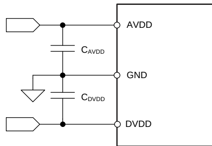
Figure 49. Power-Supply Decoupling
