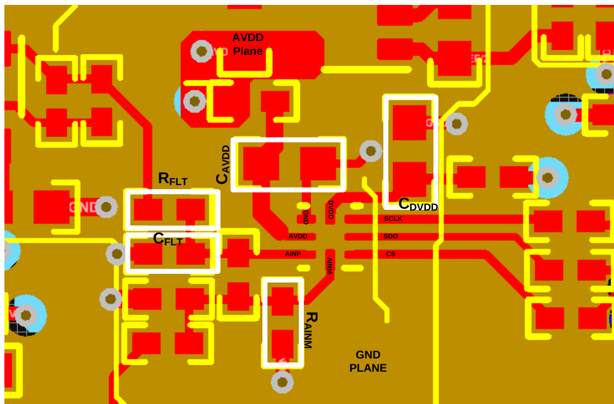
Figure 51. Example Layout
