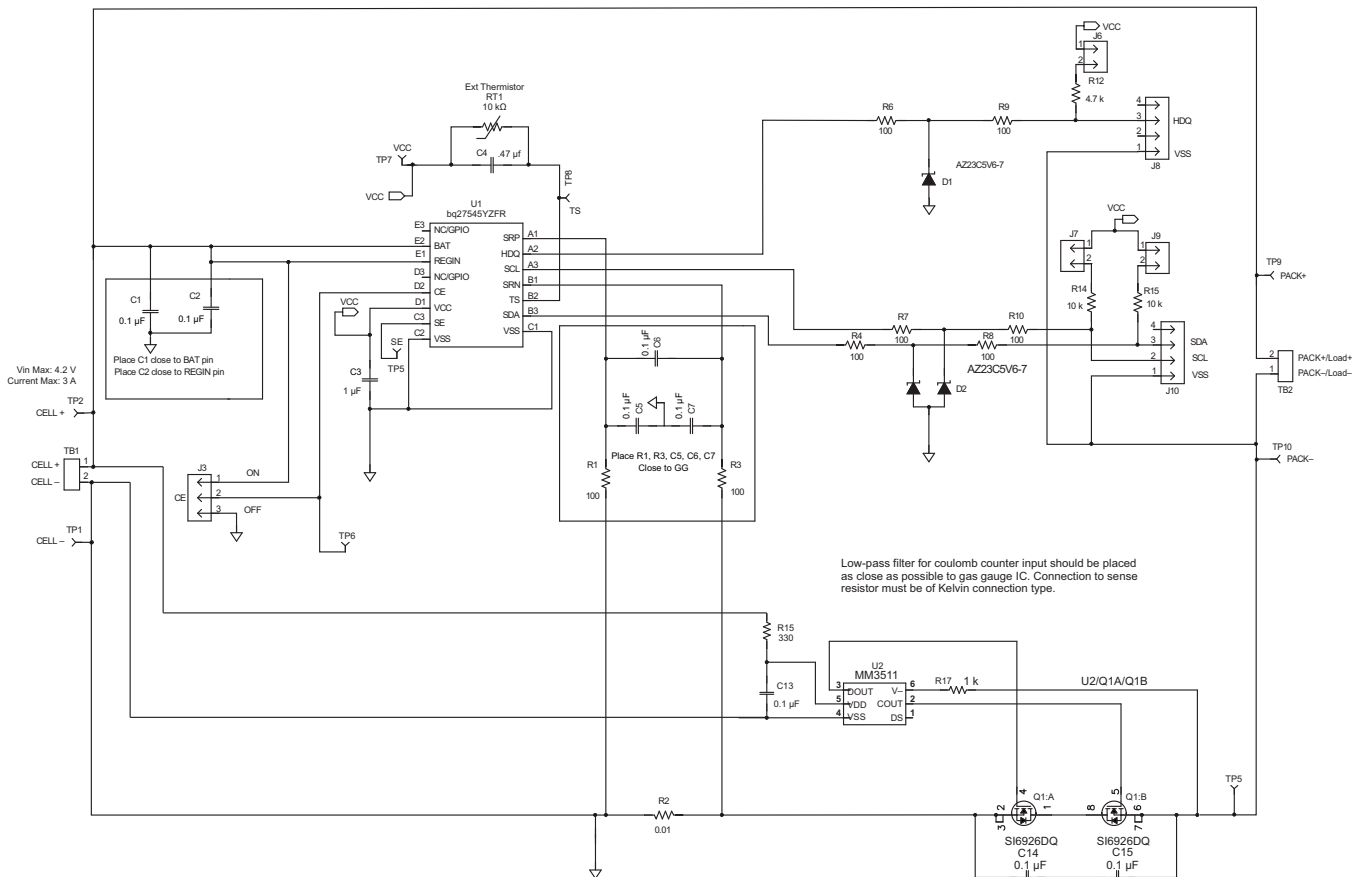
Figure 9. Reference Schematic
