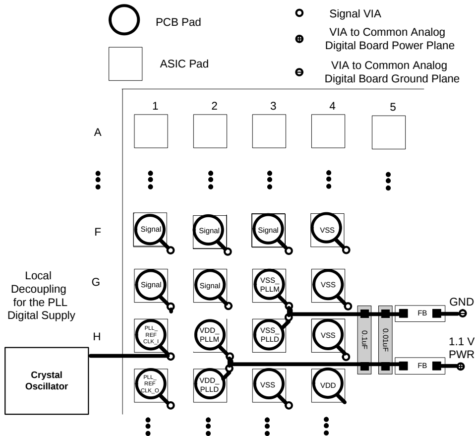
Figure 27. PLL Filter Layout
