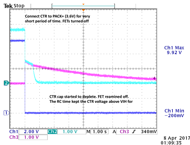
Figure 21. Setup CTR for System Reset (Using 5 M \Omega and 1 \mu F RC)
