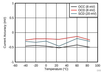
Figure 4. Overcurrent Accuracy Across Temperature
