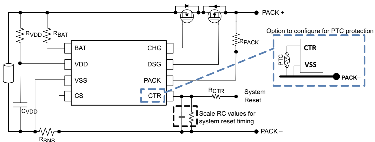
Simplified Schematic
