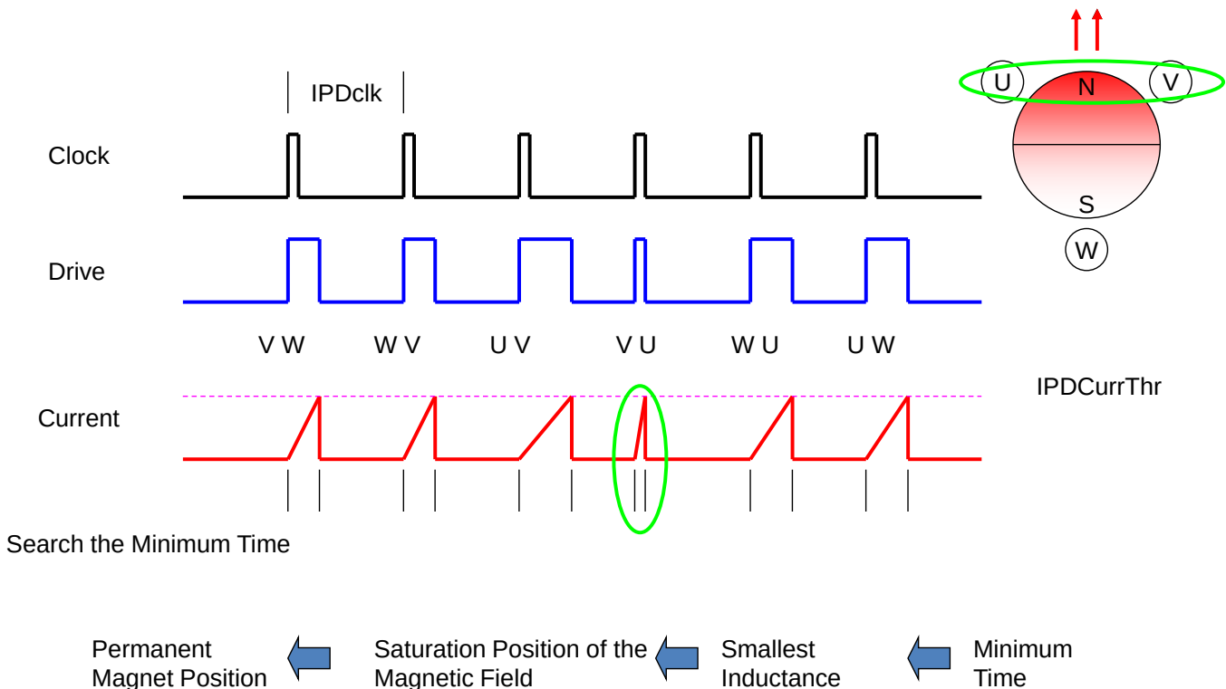
Figure 20. IPD Function
