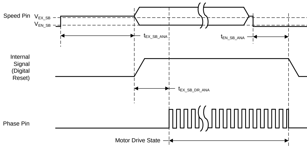
Figure 3. DRV10987S Analog Mode Timing
