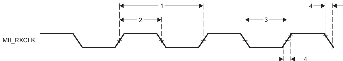
Figure 7-108. PRU-ICSS MII[x]_RXCLK Timing
