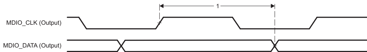
Figure 7-107. PRU-ICSS MDIO_DATA Timing - Output Mode
