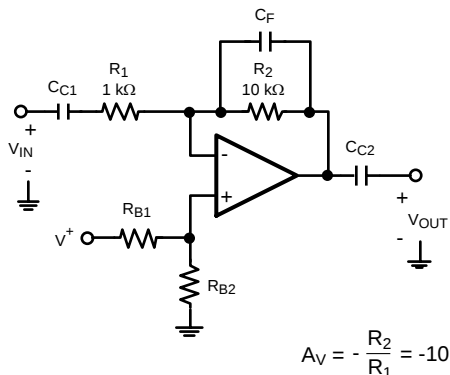
Figure 57. Inverting Audio Preamplifier
