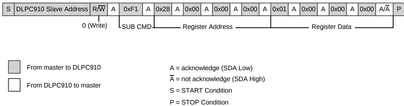
Figure 6. Example I2C Master Writing DLPC910 Register Data
