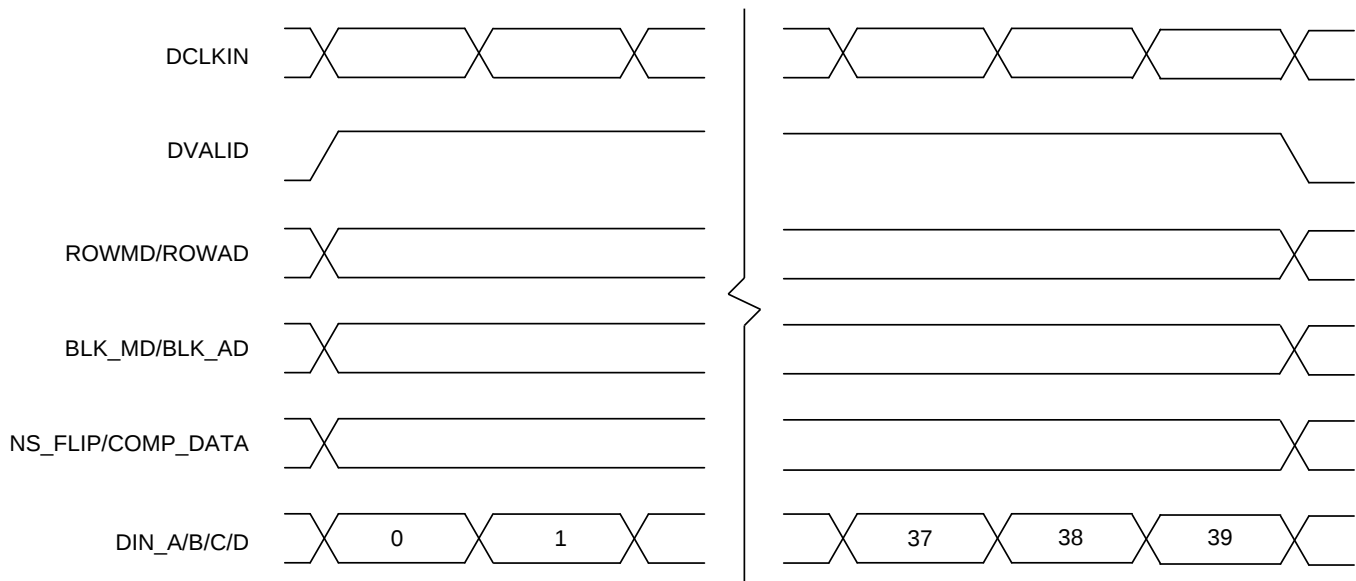
Figure 8. DLP9000X Single Row Write Operation
