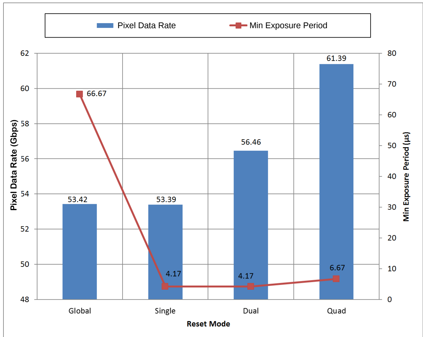
Figure 17. DLP9000X Performance Plot at 480 MHz DDC_DCLK
