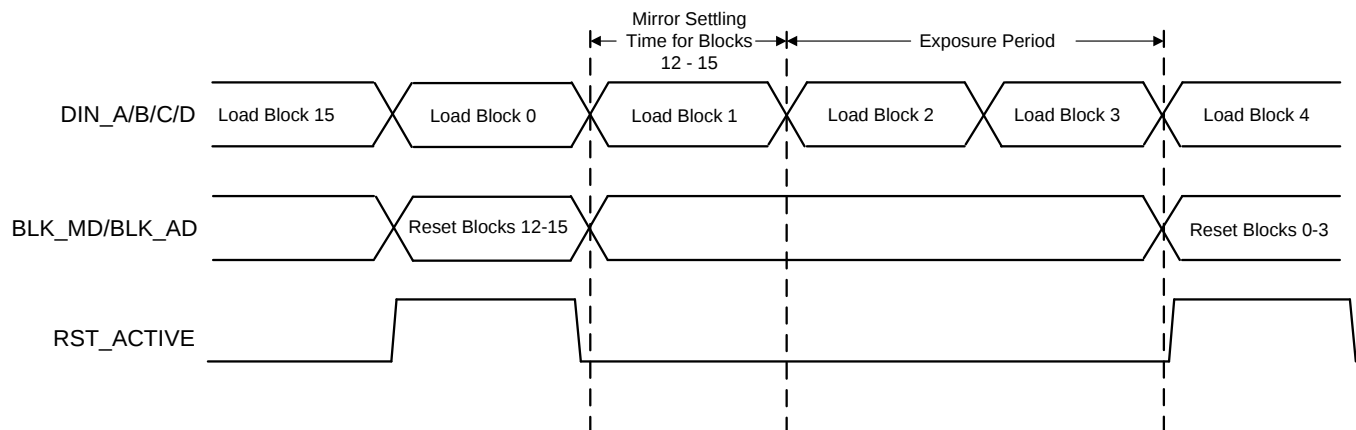
Figure 13. Quad Block Load Phased Sequence
