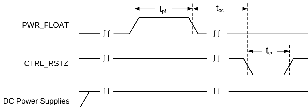
Figure 21. Restart Without Removing Power
