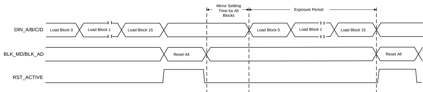
Figure 14. Full DMD Global Load Sequence
