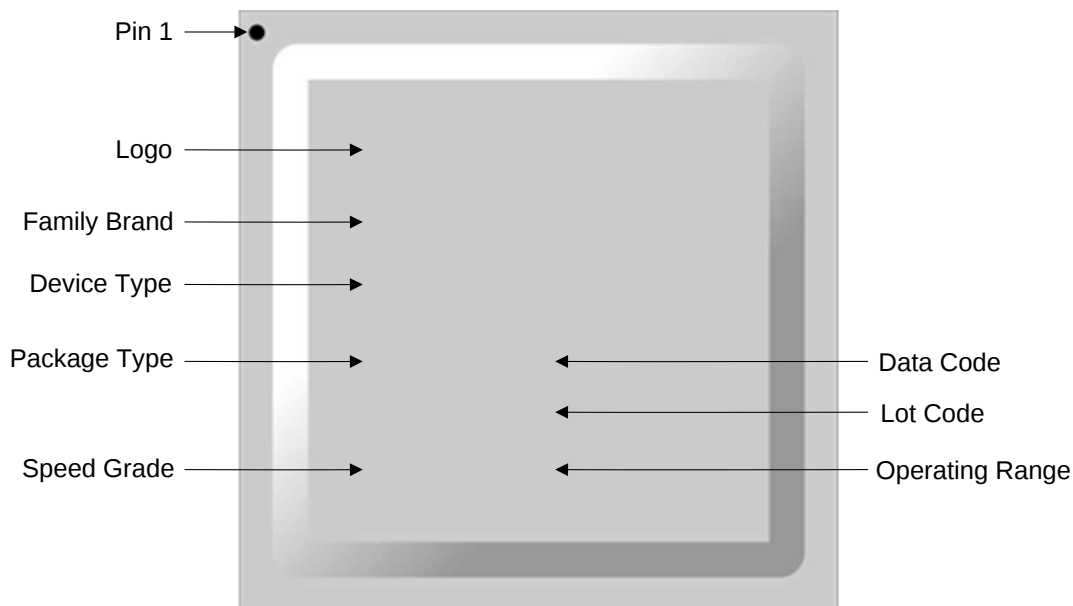
Figure 23. DLPC910 Device Markings
