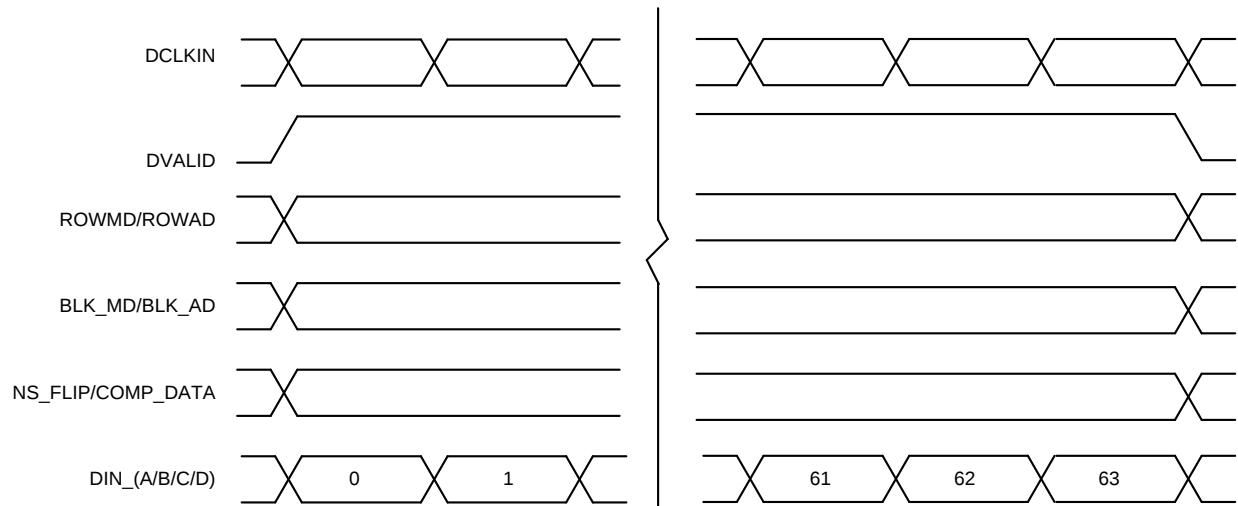
Figure 9. DLP6500 Single Row Write Operation
