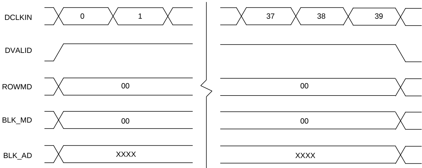
Figure 10. DMD No-op Row Cycle
