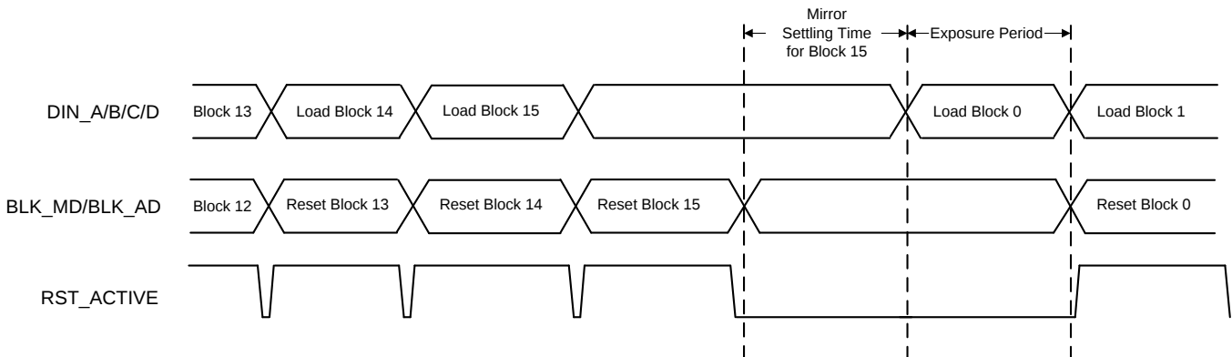
Figure 11. Single Block Load Phased Sequence
