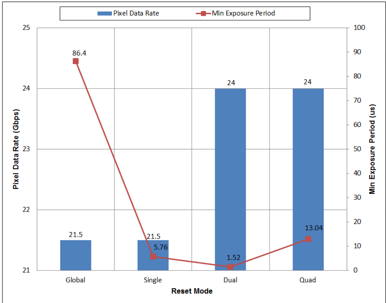
Figure 18. DLP6500 Performance Plot at 400 MHz DDC_DCLK
