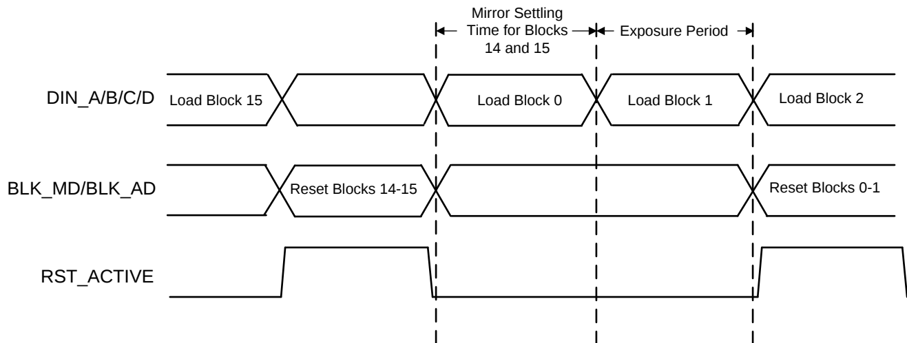
Figure 12. Dual Block Load Phased Sequence
