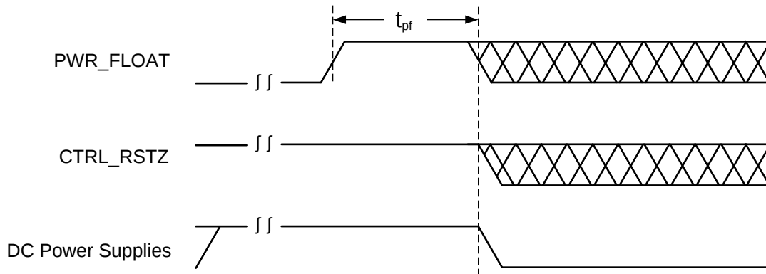
Figure 20. Removing Power After Asserting PWR_FLOAT
