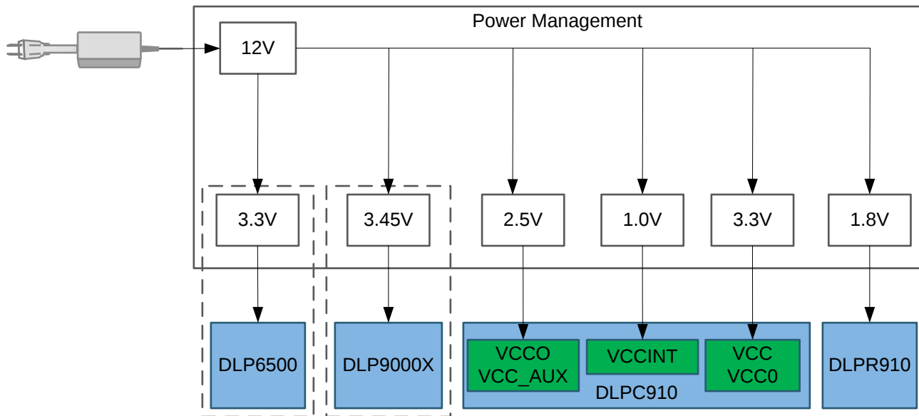
Figure 19. Power Distribution
