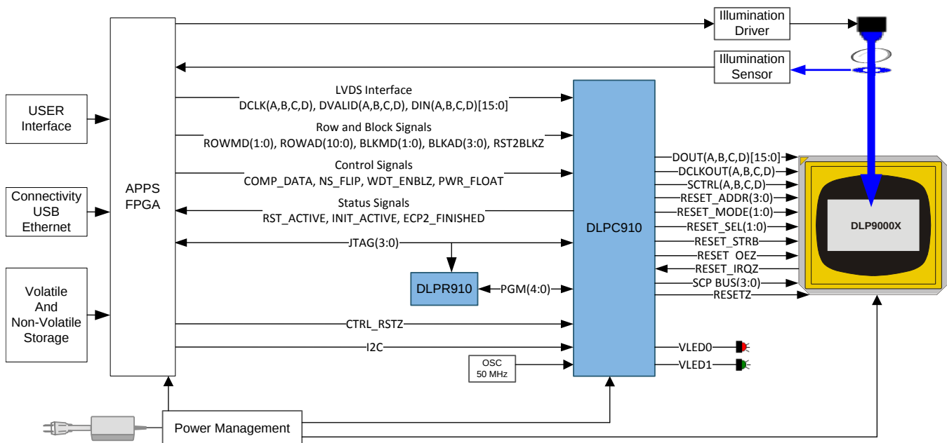
Figure 15. Typical DLP9000X High Speed Application
