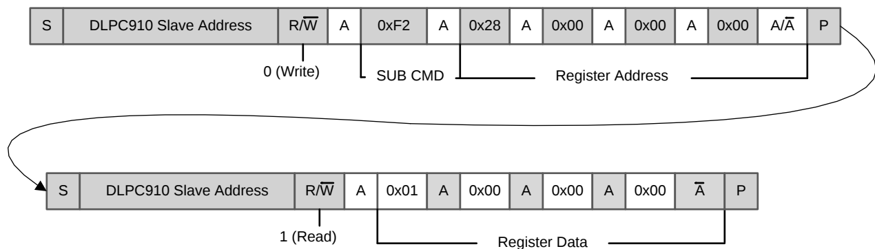
Figure 7. Example I2C Master Reading DLPC910 Register Data
