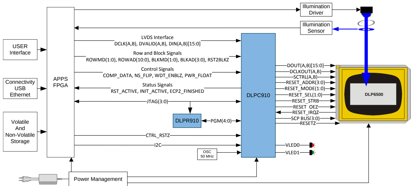
Figure 16. Typical DLP6500 High Speed Application
