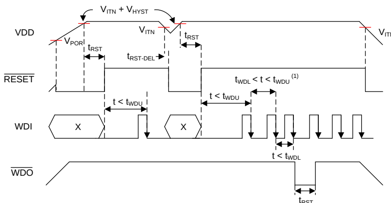
Figure 1. Timing Diagram
