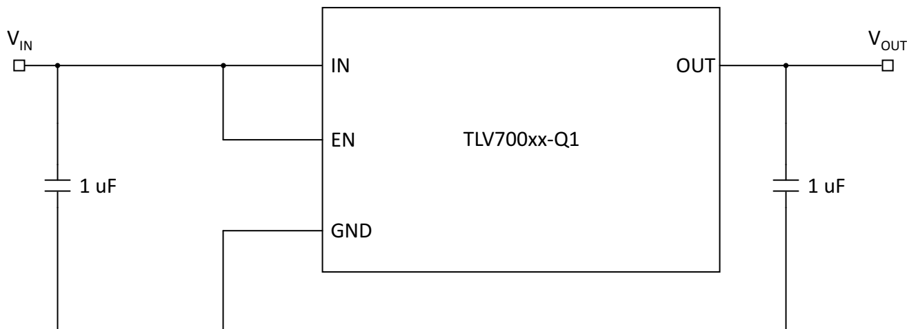
Figure 21. Simplified Schematic
