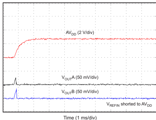
Figure 85. Power-On Glitch Reset to Zero Scale
