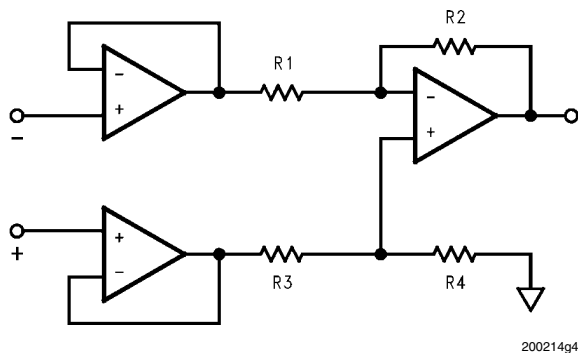
FIGURE 5. Rail-to-rail instrumentation amplifier
