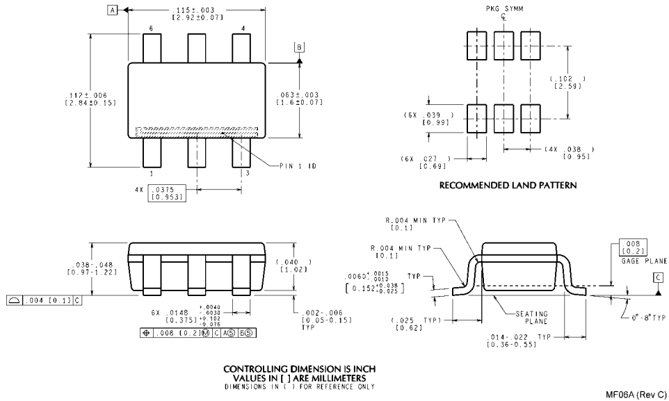
6-Pin SOT23 NS Package Number MF06A
