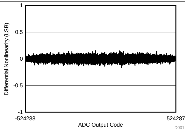
Figure 6. Typical DNL
