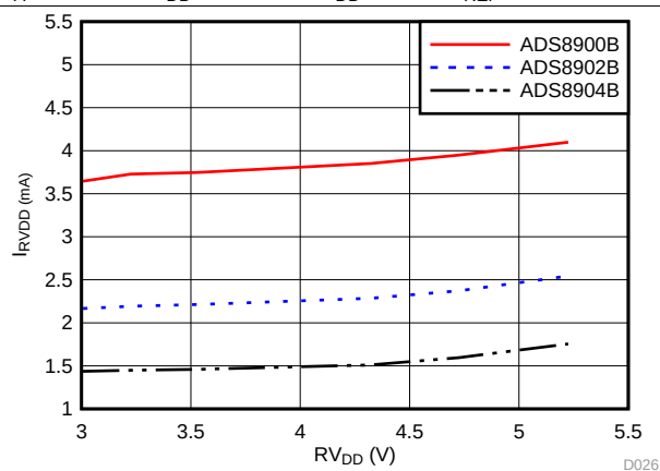
Figure 30. Analog Supply Current vs Supply Voltage
