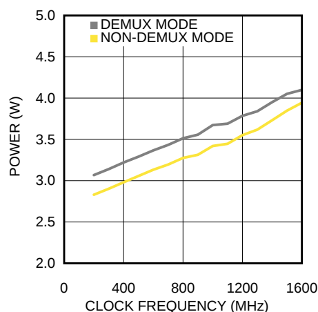
Figure 4-34. Power Consumption vs Clock Frequency (ADC12D1600RF)
