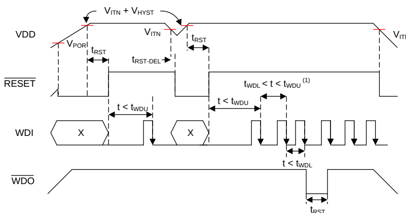
Figure 1. Timing Diagram
