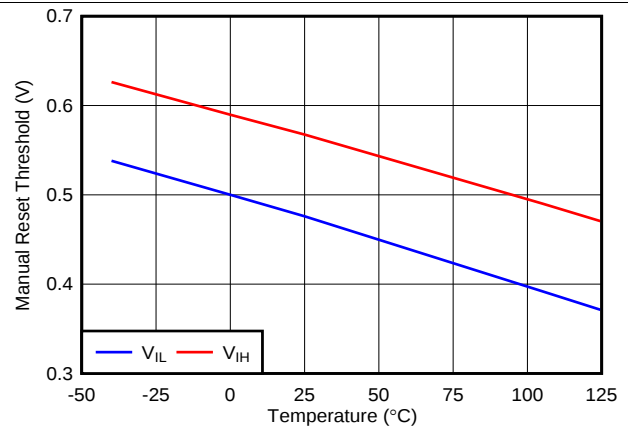
Figure 4. \overline{MR} Threshold vs Temperature
