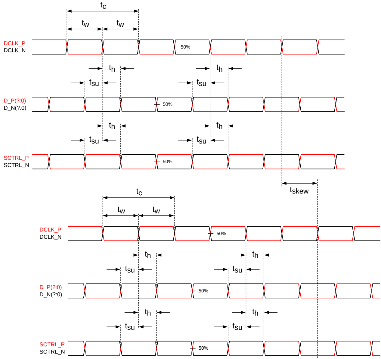
Figure 6. Timing Requirements
