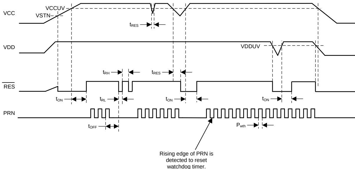
Figure 1. Watchdog Timing Chart
