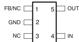
DCK PACKAGE SC70-5 (TOP VIEW)
