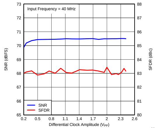
Figure 23. Performance vs Clock Amplitude
