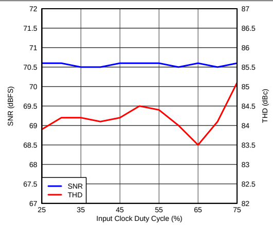
Figure 25. Performance vs Clock Duty Cycle
