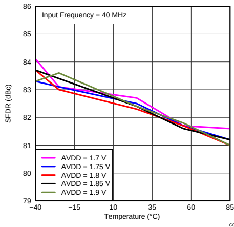
Figure 20. SFDR vs AVDD Supply and Temperature
