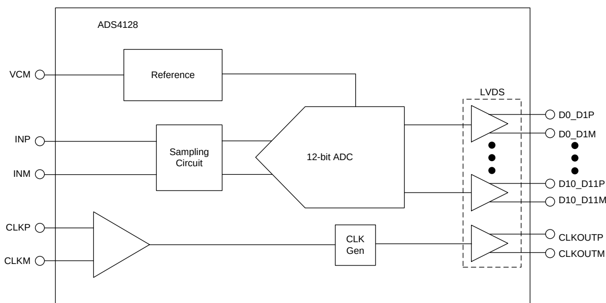
ADS4128 Block Diagram
