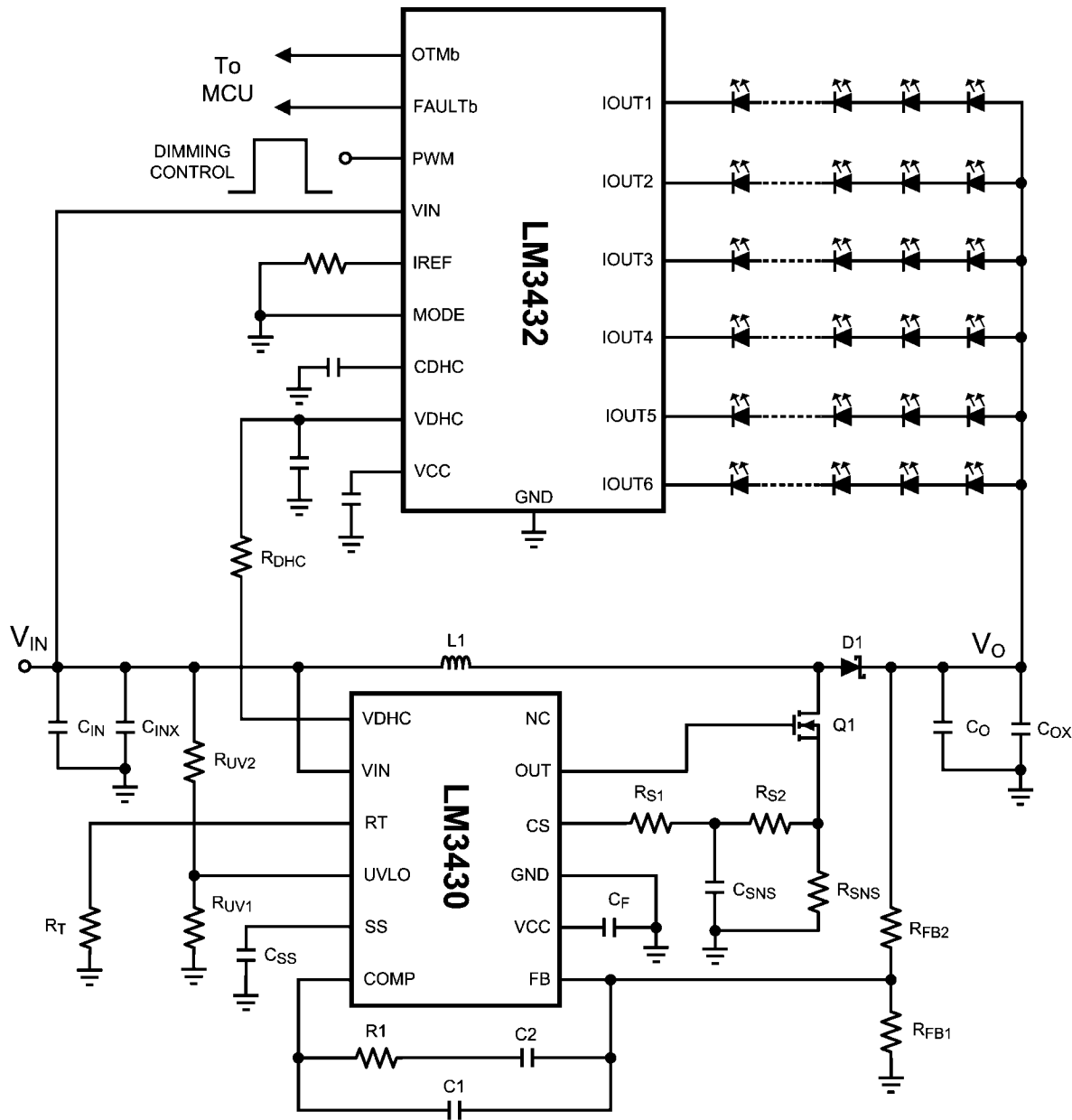
FIGURE 1. LM3430 with LM3432
