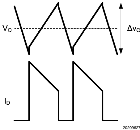
FIGURE 6. \Delta V_O Using Low ESR Capacitors
