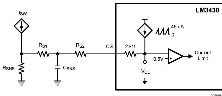
FIGURE 4. Slope Compensation
