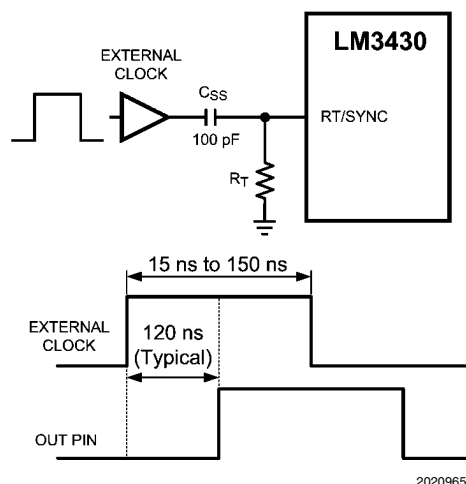
FIGURE 3. Sync Operation
