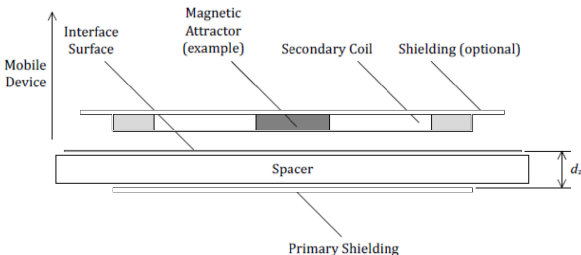
Figure 31. WPC v1.0 Receiver Coil Test Fixture for the Inductance Measurement L_s' (copied from System Description Wireless Power Transfer, volume 1: Low Power, Part 1 Interface Definition, Version 1.0.1, Figure 4-4)
