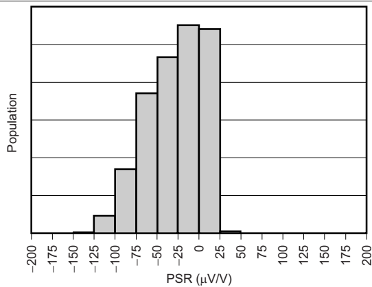
Figure 31. Voltage Reference Power-Supply Rejection Production Distribution
