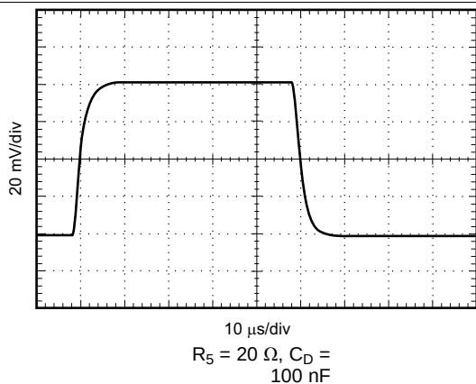
Figure 44. Figure 44 Performance ( V_{OUT} )
