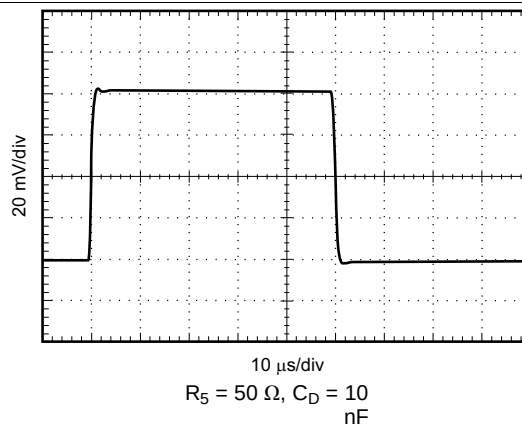
Figure 45. Figure 45 Performance ( V_{OUT} )
