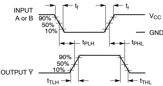
Figure 4. Switching Waveforms
