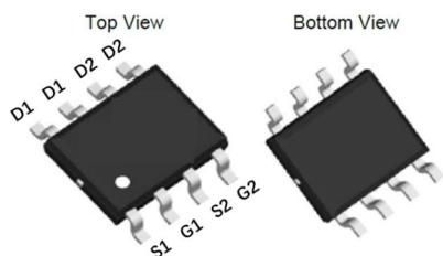
SOP-8 Dual
