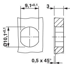
Dimensional drawing
