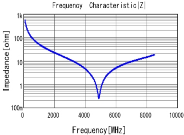
■ GJM1555C1H3R0WB01 |Z| DC0V, 25degC
