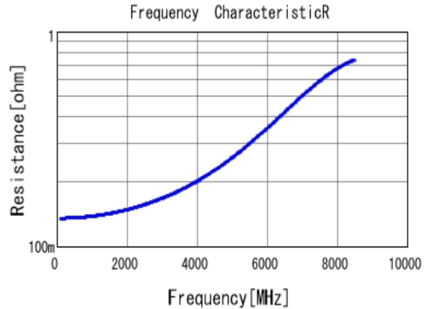
■ GJM1555C1H3R0WB01 R DC0V, 25degC
