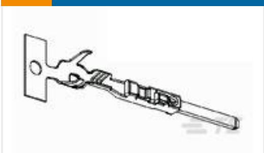
TE Part #2141114-3 MCON 1.2 CB TAB SWS AG
