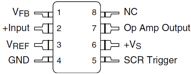
Figure 2. Pin Assignment
