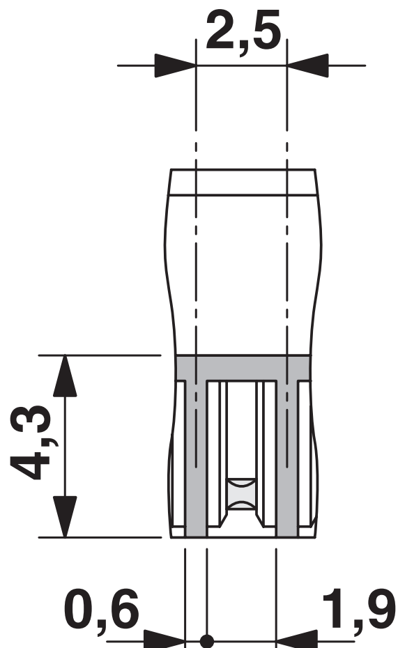
Dimensional drawing
