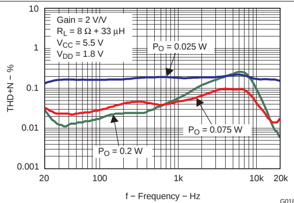
Figure 18. Total Harmonic Distortion + Noise vs Frequency
