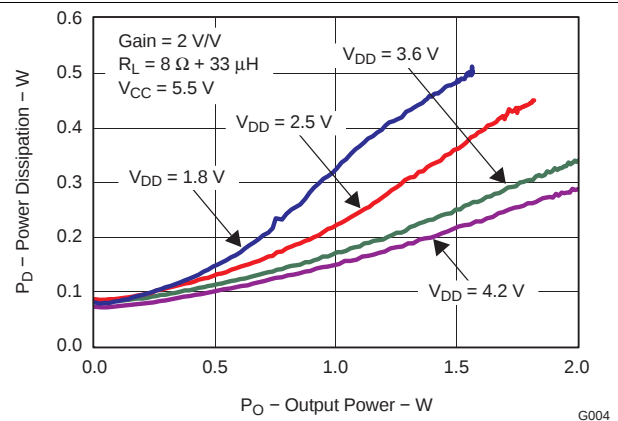
Figure 4. Power Dissipation vs Output Power
