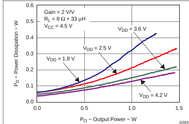
Figure 3. Power Dissipation vs Output Power
