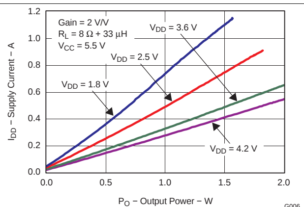
Figure 6. Supply Current vs Output Power
