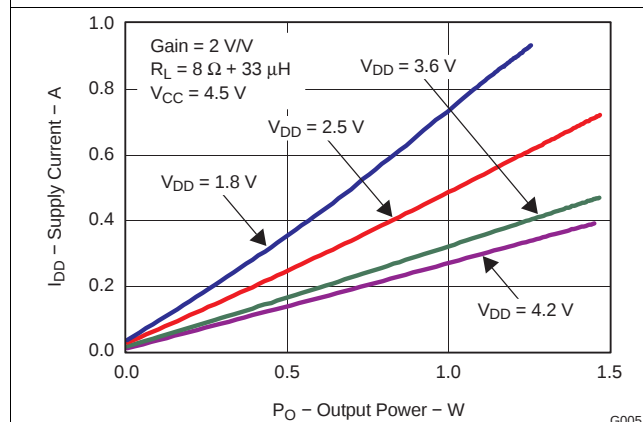
Figure 5. Supply Current vs Output Power
