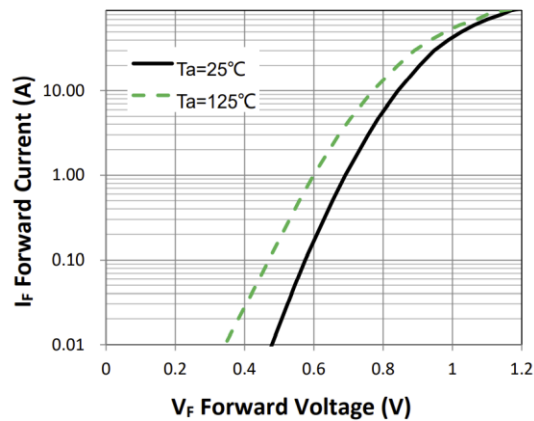
Figure 1. Forward Characteristic(typ.)
