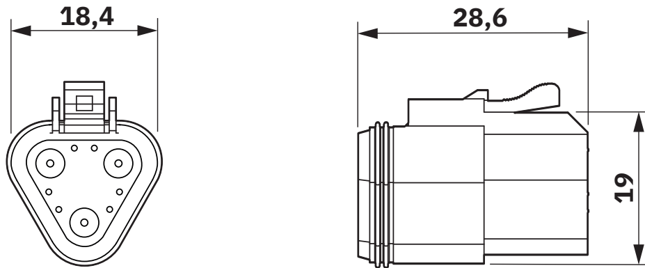
Dimensional drawing
