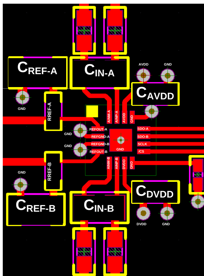
Figure 52. Example Layout for the ADS7251 and ADS7851
