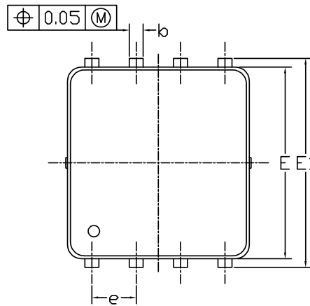
DFN5x6_8L_EP1_P PACKAGE OUTLIN
