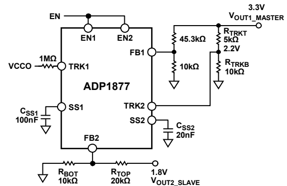
Figure 38. A Simple Ratiometric Tracking Circuit (Slave Channel Has a Faster Ramp Rate)
