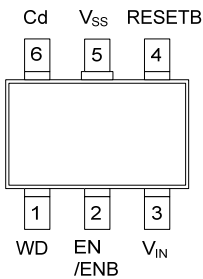
SOT-26 (TOP VIEW)
