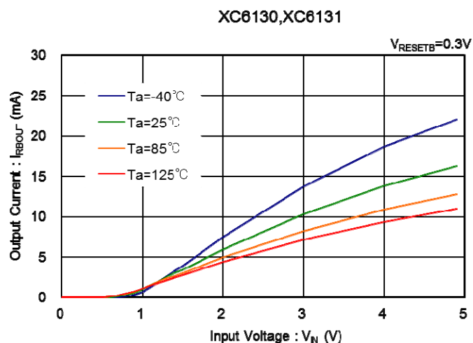
(5) Output Current vs. Input Voltage
