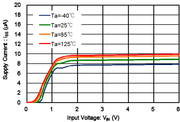
XD6130 ( V_{DF(T)}=1.6V )
