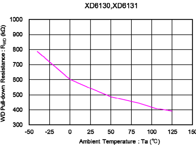
(21) WD Pull-down Resistance vs. Ambient Temperature
