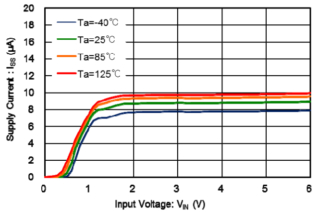
XD6130 ( V_{DF(T)}=3.0V )
