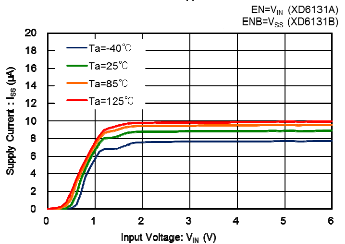
XD6131 ( V_{DF(T)}=5.0V )
