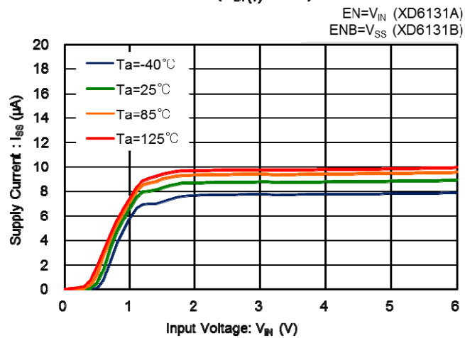
XD6131 ( V_{DF(T)}=3.0V )
