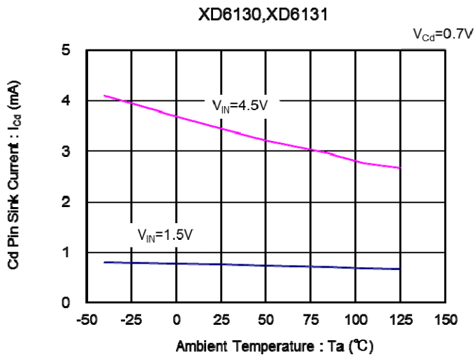
(7) Release Delay Time1 vs. Ambient Temperature
