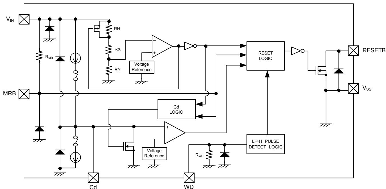
XD6130 Series
