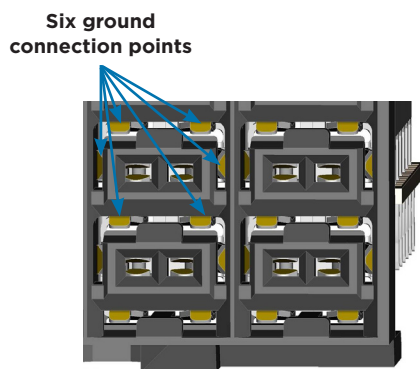
Fig. 1. Close up of signal contacts
