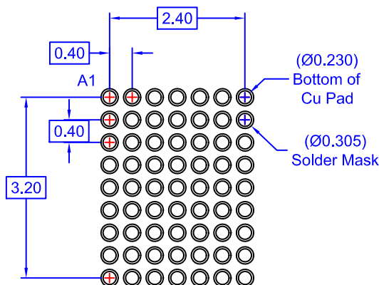
RECOMMENDED LAND PATTERN (NSMD TYPE)
