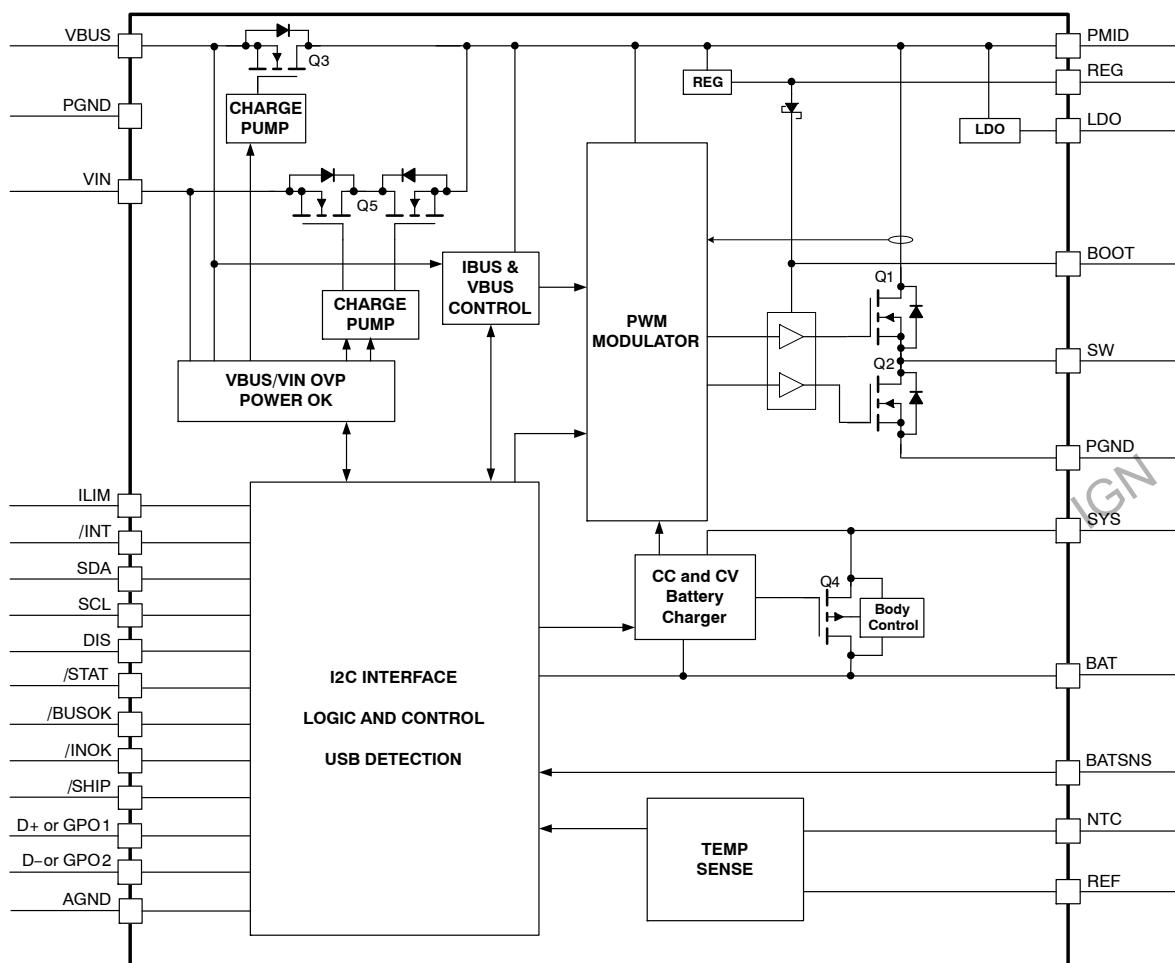
Figure 5. Block Diagram
