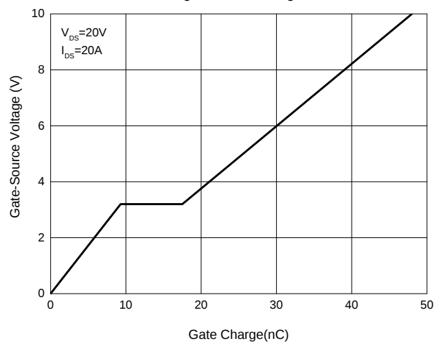
Fig. 6 - Gate Charge
