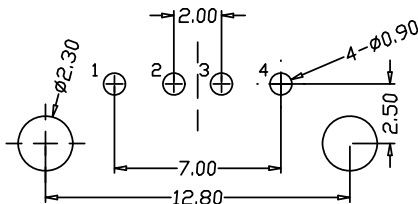
PCB LAYOUT
