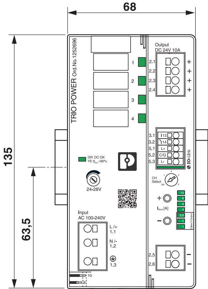
Dimensional drawing
