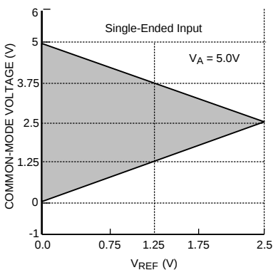
Figure 60. V_{CM} range for single-ended operation
