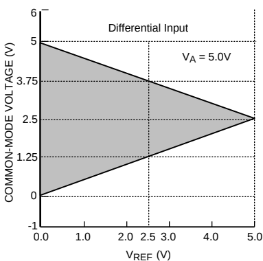
Figure 59. V_{CM} range for Differential Input operation
