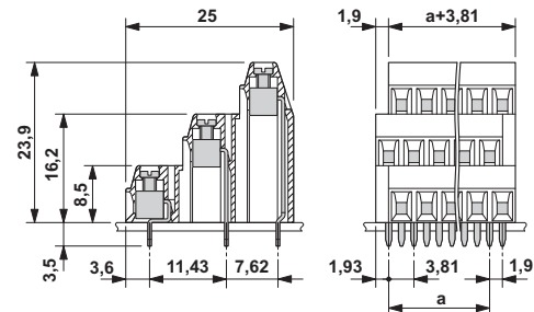
Dimensional drawing
